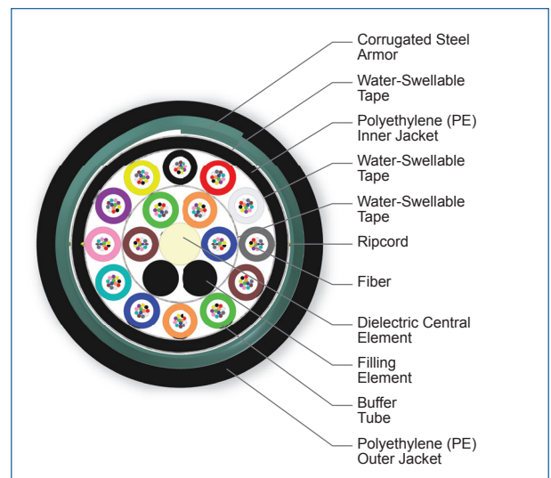
Cross Section of Part Number: 192TU5-T4131F20
