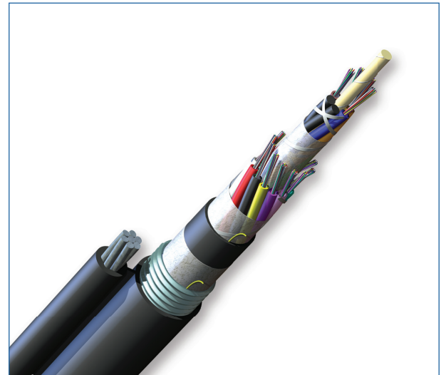
Part Number: 192TUB-T4131D20
