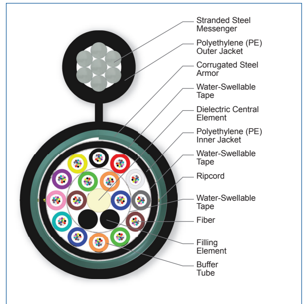
Cross Section of Part Number: 192TUB-T4131D20
