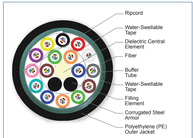
Cross Section of Part Number: 192TUC-T4131D20
