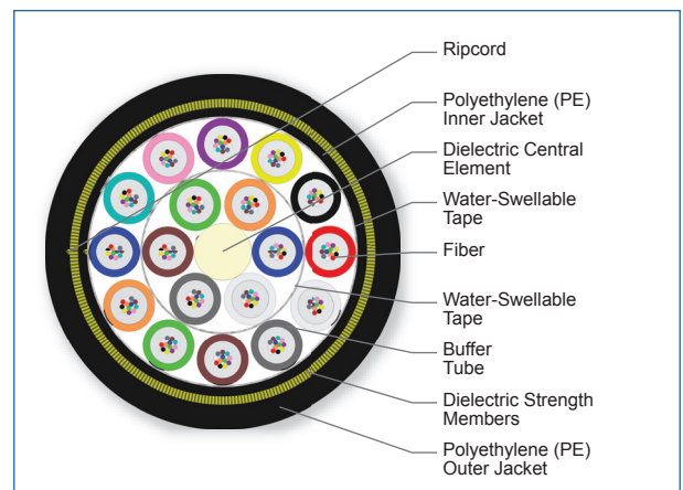
Cross Section of Part Number: 216EAE-T4201A20
