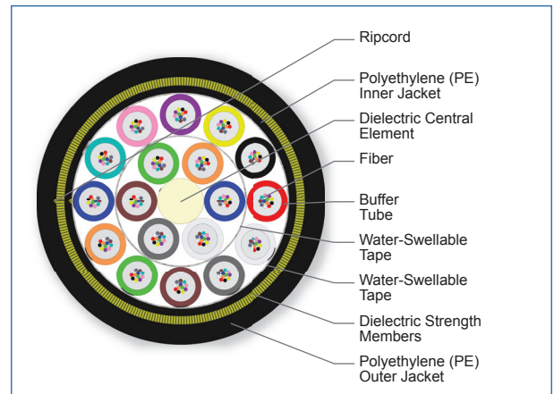
Cross Section of Part Number: 216EAE-T4401A20
