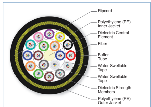
Cross Section of Part Number: 216EAE-T4A01A20
