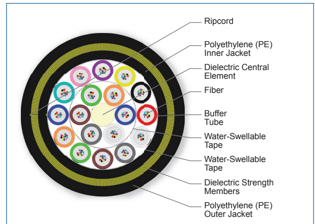
Cross Section of Part Number: 216EAE-T4B01A20
