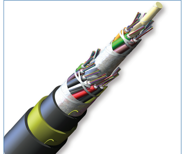
Part Number: 216EAE-T4B01A20
