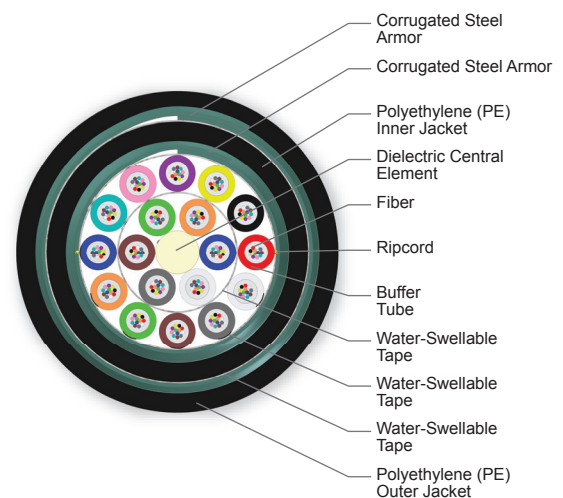
Cross Section of Part Number: 216EUD-T4101A20
