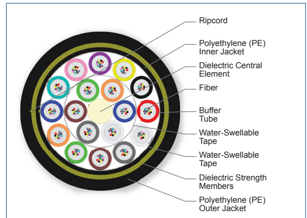
Cross Section of Part Number: 216KAE-T4430A20
