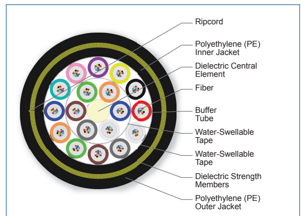
Cross Section of Part Number: 216KAE-T4830A20
