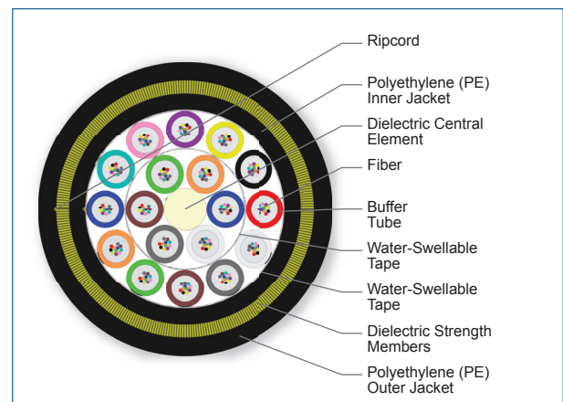
Cross Section of Part Number: 216KAE-T4B30A20
