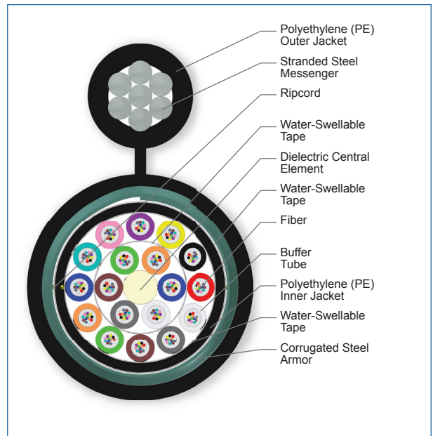
Cross Section of Part Number: 216KUB-T4130A20
