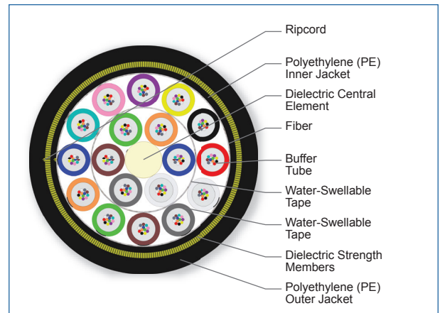
Cross Section of Part Number: 216TAE-T4231A20
