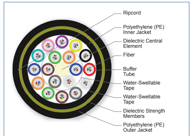
Cross Section of Part Number: 216TAE-T4831A20
