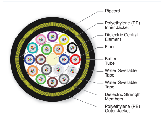
Cross Section of Part Number: 216TAE-T4B31A20
