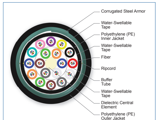
Cross Section of Part Number: 216TU5-T4131F20
