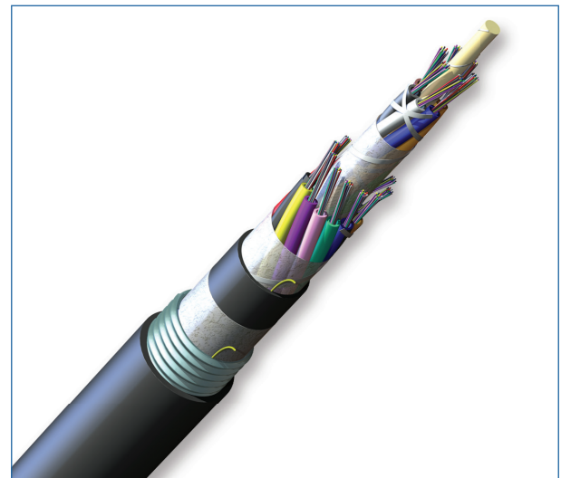
Part Number: 216TU5-T4131F20
