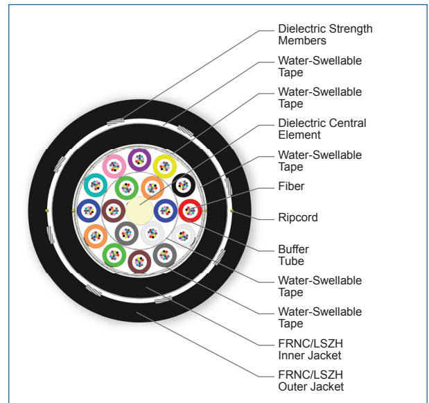
Cross Section of Part Number: 216TUL-T4691D2N
