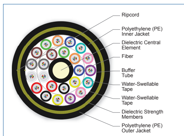
Cross Section of Part Number: 288EAE-T4A01A20
