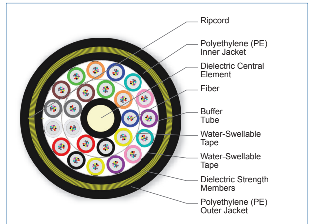
Cross Section of Part Number: 288EAE-T4C01A20
