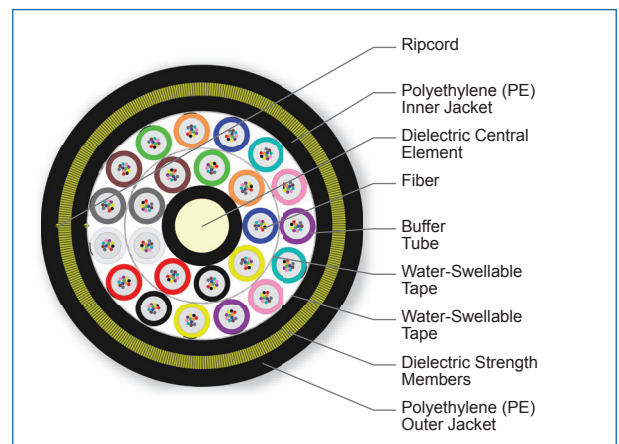
Cross Section of Part Number: 288EAE-T4E01A20
