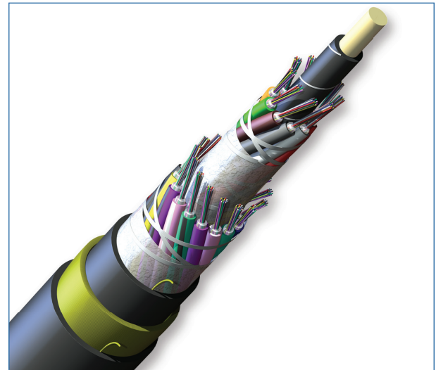
Part Number: 288EAE-T4E01A20
