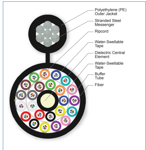
Cross Section of Part Number: 288EUA-T4101D20
