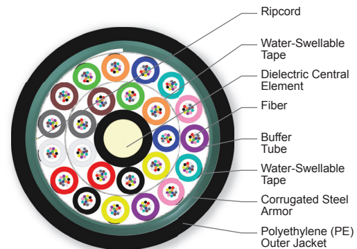
Cross Section of Part Number: 288EUC-T4100D20
