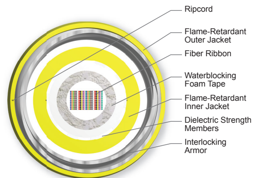
Cross Section of Part Number: 288EV7-14101DA1
