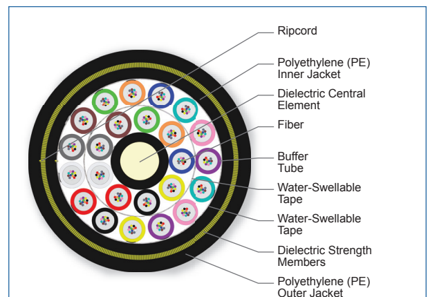
Cross Section of Part Number: 288KAE-T4630A20
