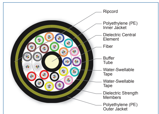
Cross Section of Part Number: 288KAE-T4C30A20
