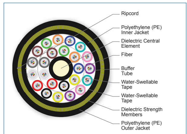
Cross Section of Part Number: 288KAE-T4E30A20
