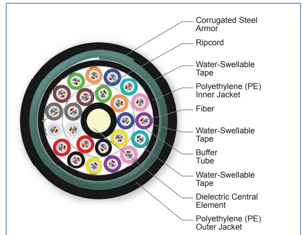
Cross Section of Part Number: 288KU5-T4130C20
