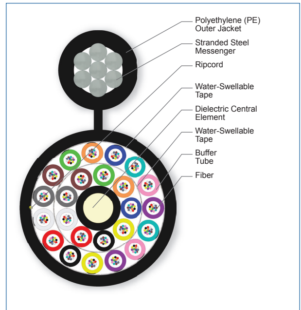
Cross Section of Part Number: 288KUA-T4130D20
