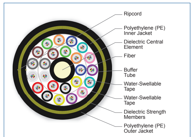
Cross Section of Part Number: 288TAE-T4A31A20
