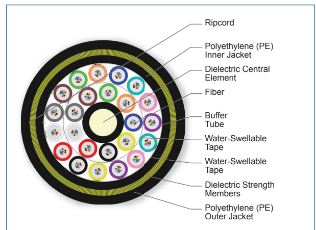
Cross Section of Part Number: 288TAE-T4C31A20
