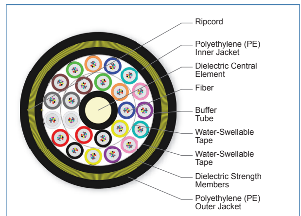
Cross Section of Part Number: 288TAE-T4E31A20
