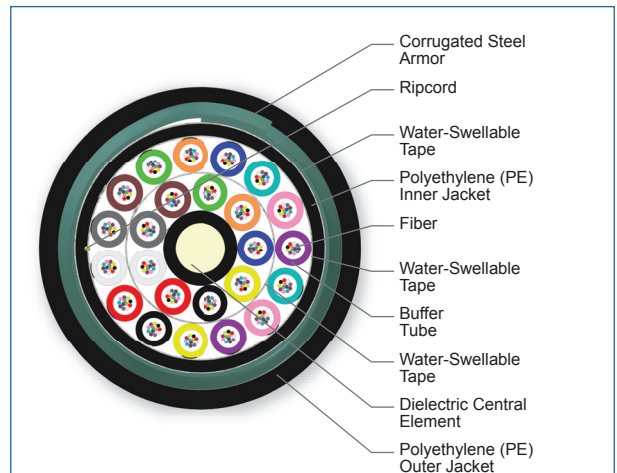
Cross Section of Part Number: 288TU5-T4131D20
