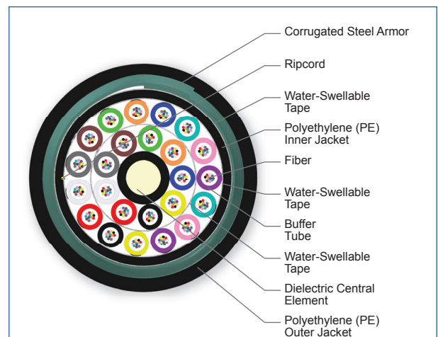
Cross Section of Part Number: 288TU5-T4131F20
