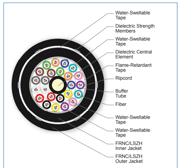
Cross Section of Part Number: 288TUL-T3690D2M
