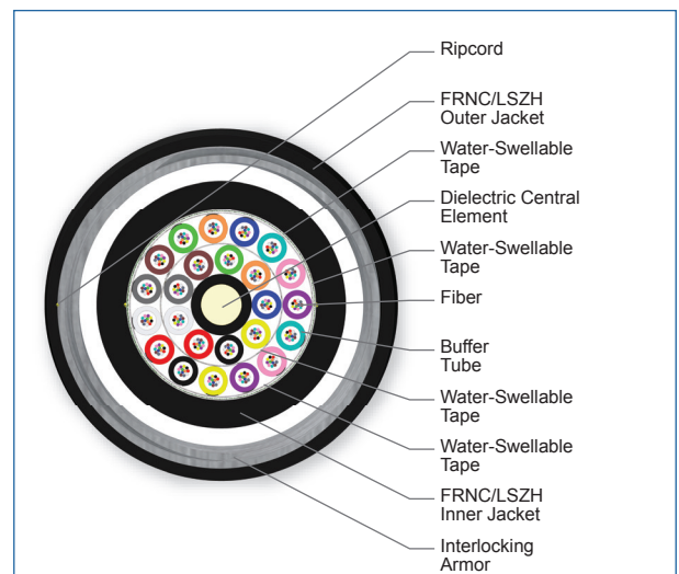
Cross Section of Part Number: 288TUZ-T4190DAN
