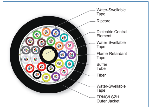
Cross Section of Part Number: 288ZUZ-T4101D2N
