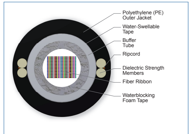
Cross Section of Part Number: 360EV4-14100D53
