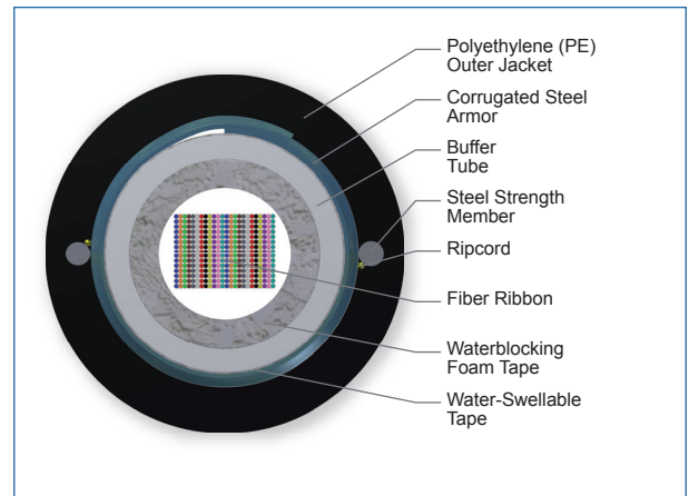
Cross Section of Part Number: 360EV5-14100D53
