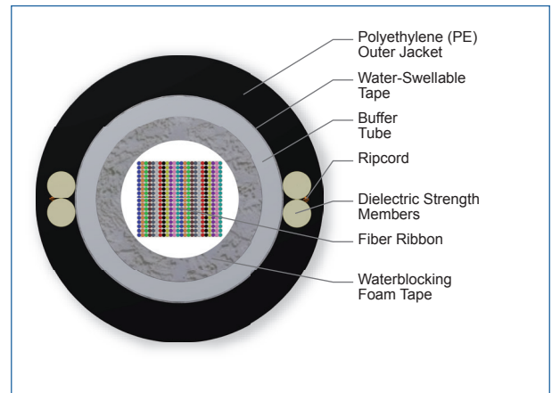
Cross Section of Part Number: 432EV4-14100D53
