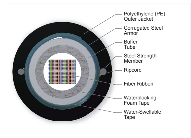
Cross Section of Part Number: 432EV5-14100D53
