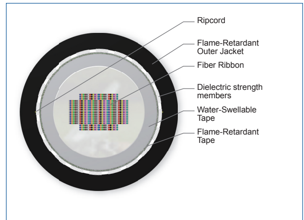
Cross Section of Part Number: 576EVF-14101-20
