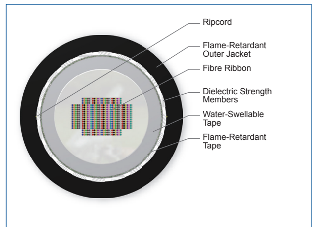
Cross Section of Order Number: 576ZVF-14101-20
