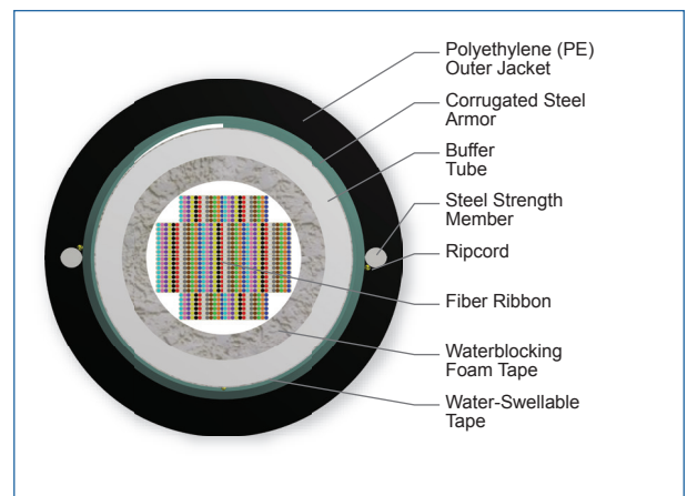
Cross Section of Part Number: 864EV5-14100D53
